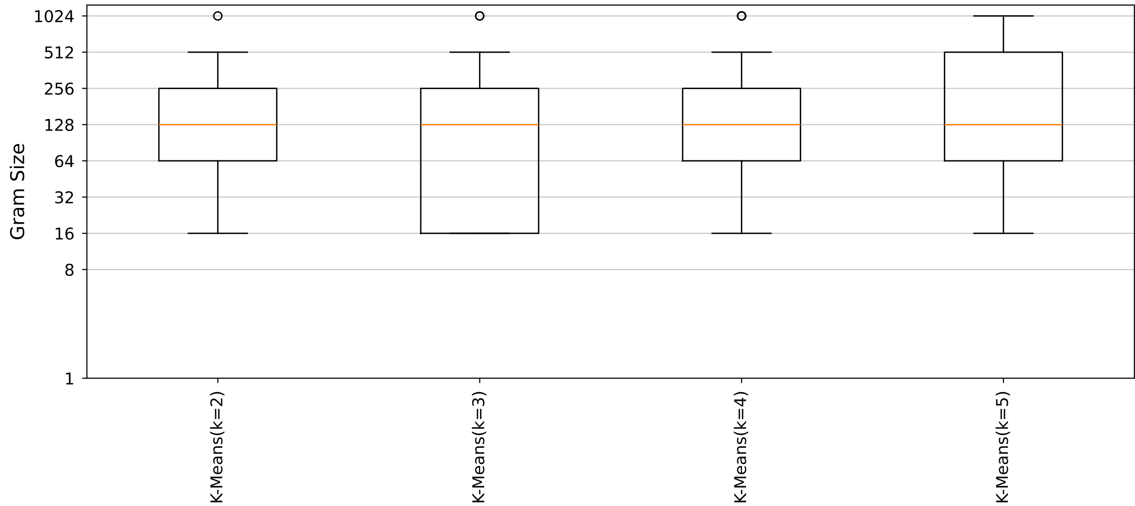
YARA Rules Gram Size Distribution (Cluster39_Size5 dataset)
